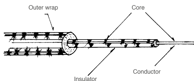
Figure 4.3: Online Cable
