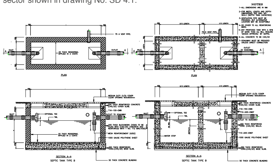
Septic Tank
